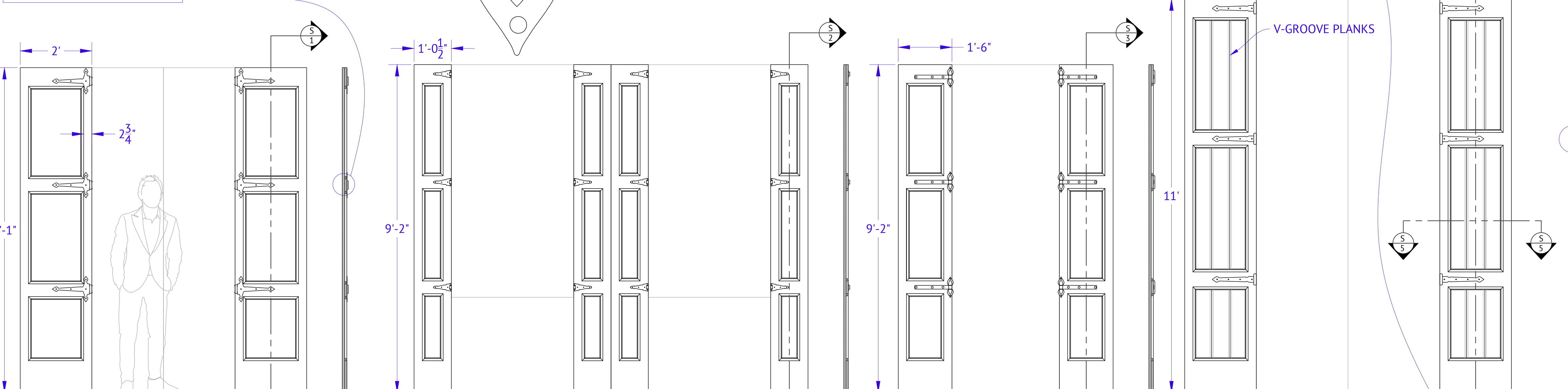
ELEVATION 1, SECTION 1 UNITS: 2 HARDWARE UNITS: 6 HARDWARE NO.: 648934 ELEVATION 2, SECTION 2 UNITS: 4 HARDWARE UNITS: 12 HARDWARE NO.: 674918 ELEVATION 3, SECTION 3 UNITS: 2 HARDWARE UNITS: 6 HARDWARE NO.: 648942 ELEVATION 4, SECTION 4 & 5 UNITS: 2 HARDWARE UNITS: 6 HARDWARE NO.: 648938
