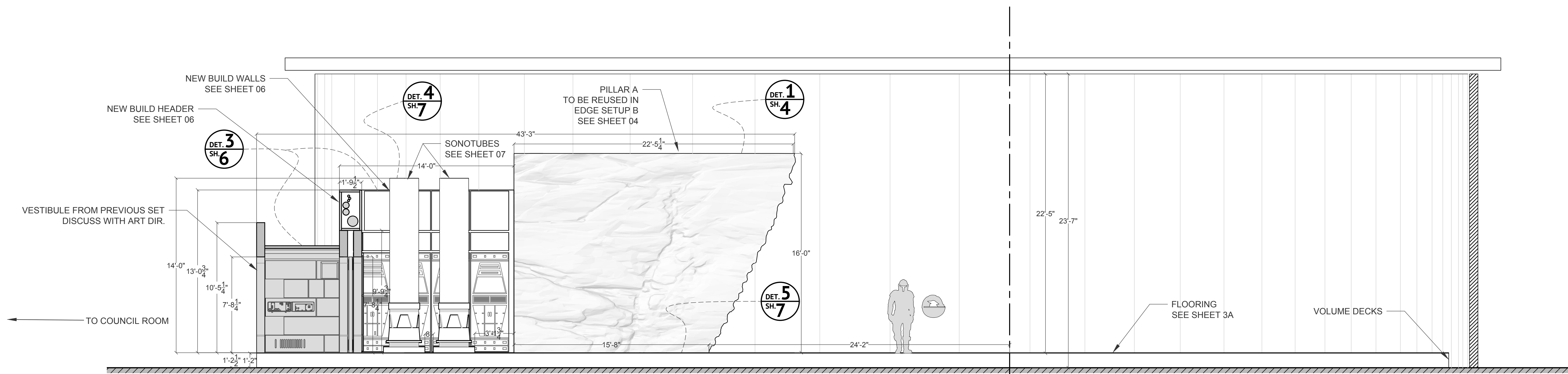
A A ELEVATION - HALLWAY SETUP (VOLUME 2A) SCALE: 1/4" = 1'-0"
