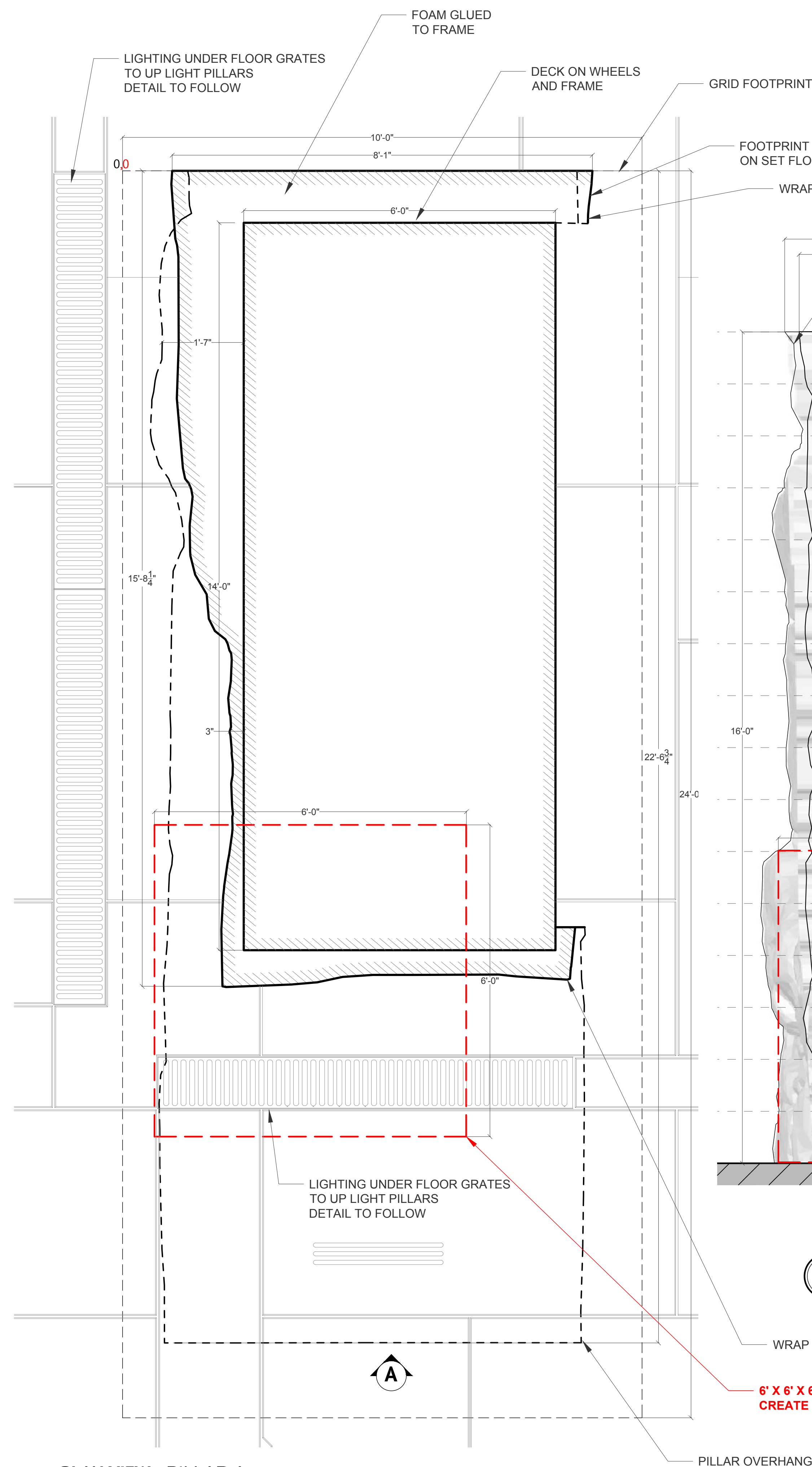
PL PLAN VIEW - PILLAR A SCALE: \frac{3}{4}'' = 1'-0''
