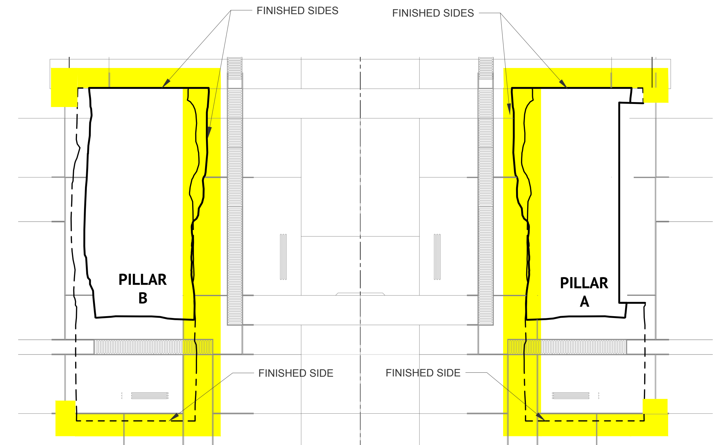
PL PLAN VIEW - PILLAR A AND B SCALE: \frac{1}{4}'' = 1'-0''
