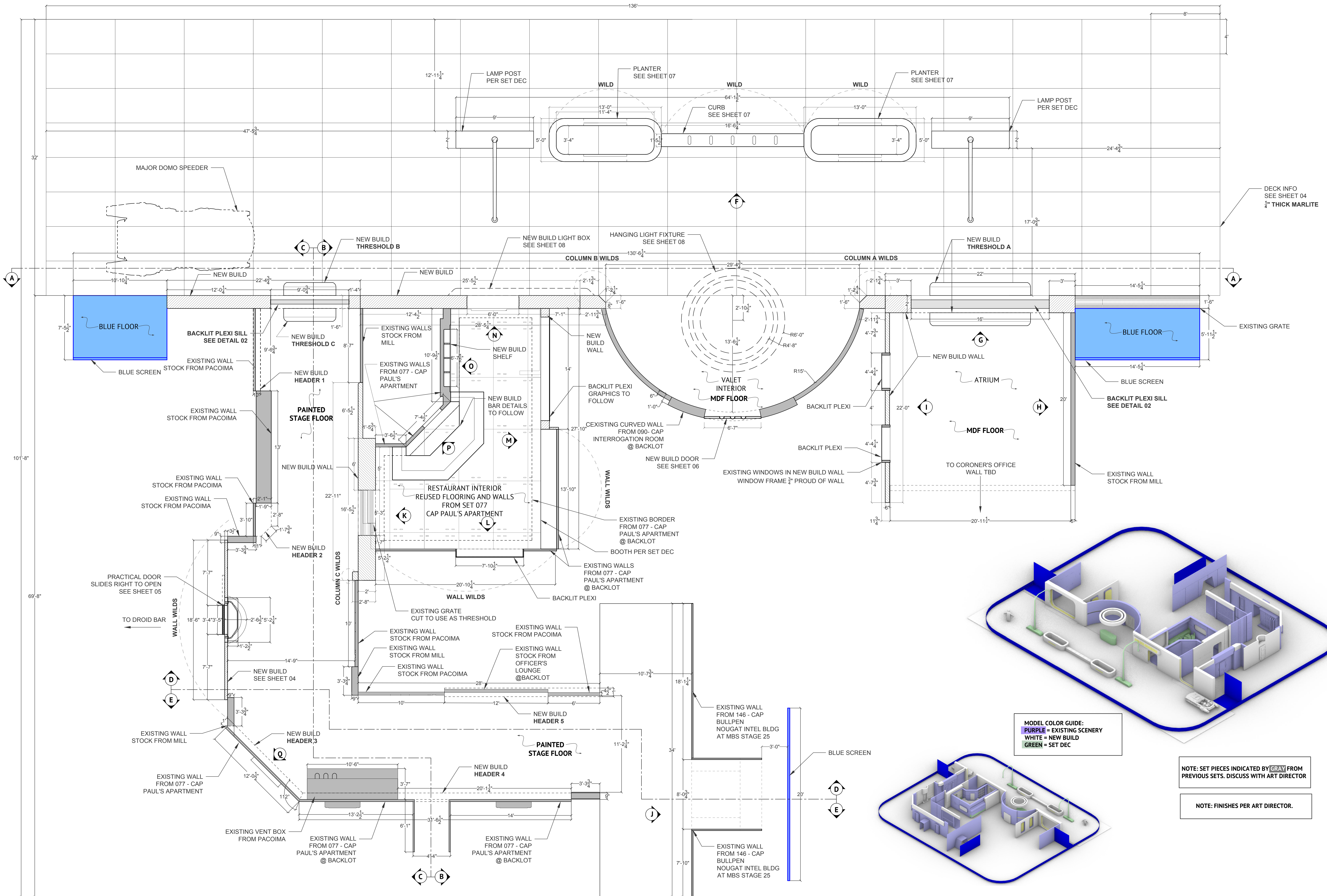
PL PLAN VIEW - SCALE: 1/4" = 1'-0"
